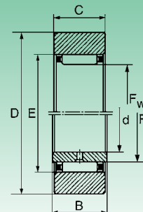
RSTO..X STO..X
